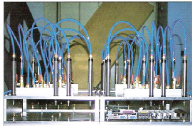
線上振動專用測試夾具 (On Line Fixture)
