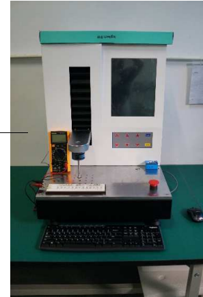
Click Lifetime Tester
