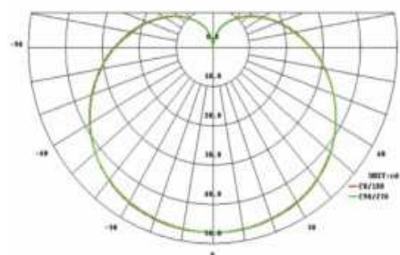
Polar Luminous Intensity Distribution
