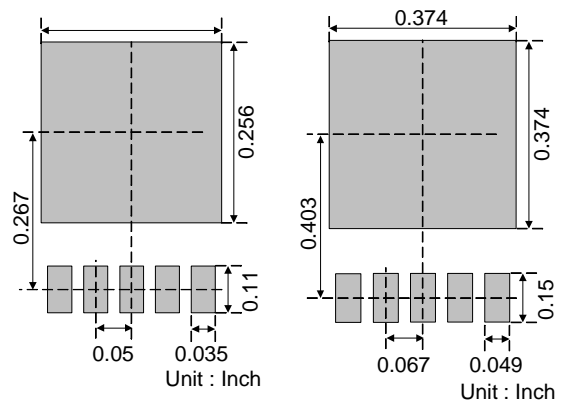
TO-252-5
