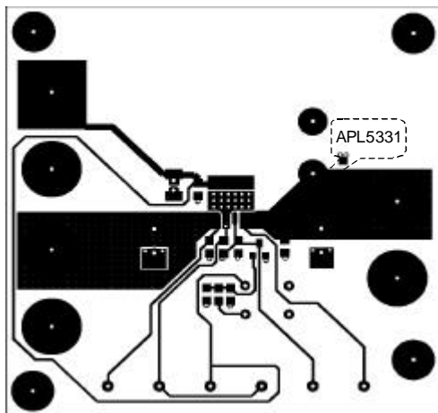
Figure 2(b) Top layer
