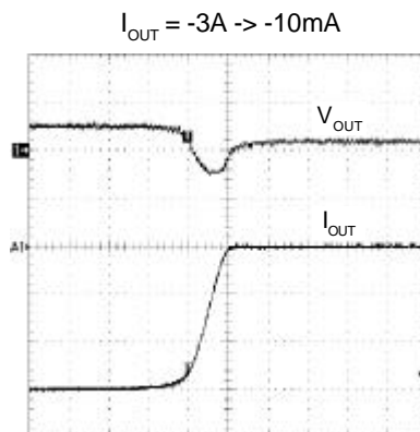
Ch1 : V_{OUT} , 20mV/Div, DC, Offset = 1.250V Ax1 : I_{OUT} , 1A/Div Time : 1 \mu s /Div
