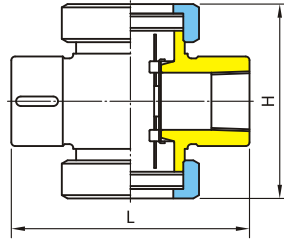
TH-10K
